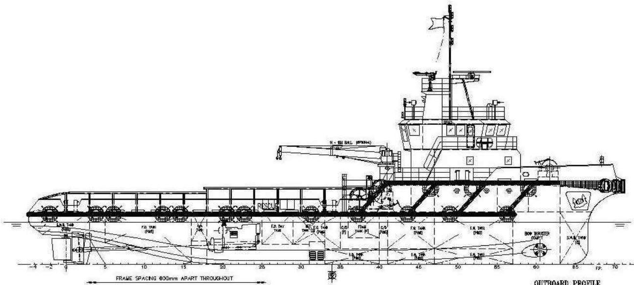
OUTBOARD PROFILE
