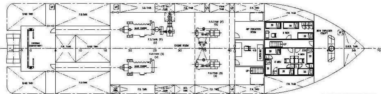
BELOW MAIN DECK PLAN
