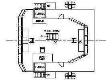
WHEELHOUSE DECK PLAN
