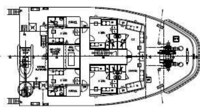
FORECASTLE DECK
