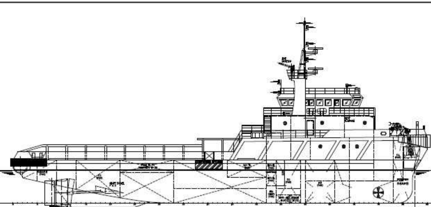
OUTBOARD PROFILE
